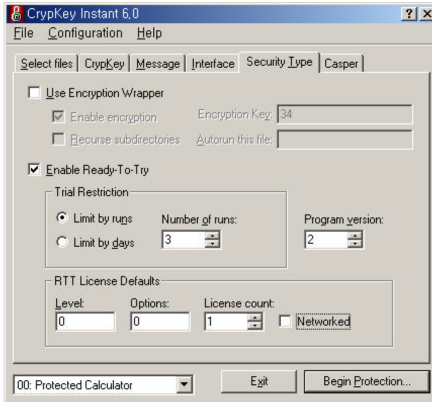
[ 69] CrypKey Instnat Security Type
